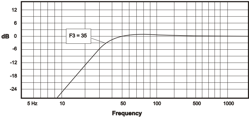
QC12S4 Amplitude Response (dB/Hz)
